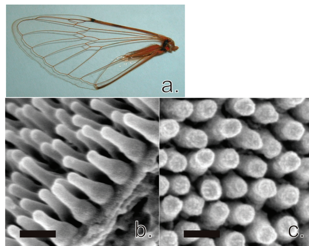
Figure 1. (a and b) Cicada wing and (c) cicada wings coated with inorganic film using ALD (20 cycles TMA/water +100 cycles DMZ/water). The scale bars are 200 nm.
